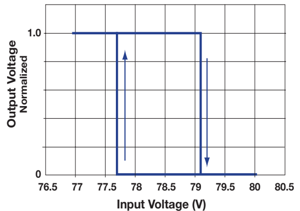
Overvoltage Hysteresis
