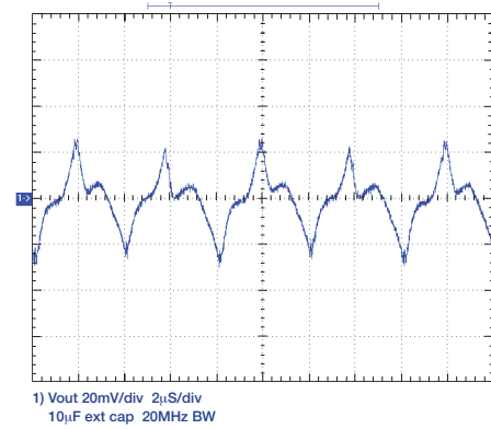
Voltage Ripple
