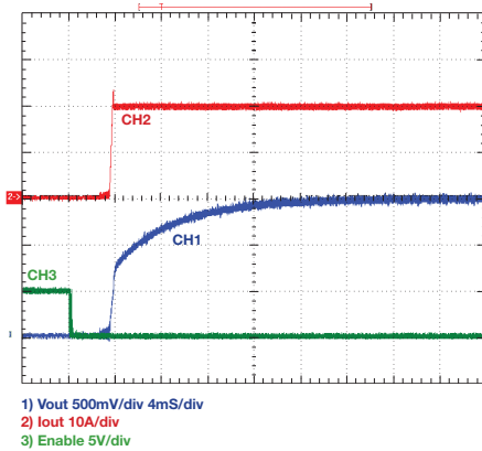
Start Up
