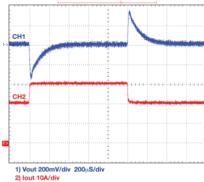
Transient Response
